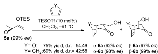
Scheme 3. Asymmetric (4+3) cycloaddition of 5a .
