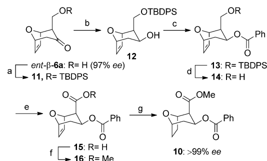
Scheme 5. Asymmetric synthesis of the DAT inhibitor 10 . Reaction conditions: a) TBDPSCl, imidazole, DMAP, CH 2 Cl 2 , 96%. b) Sml 2 , i PrOH, MeCN, 87%, d.r. = 7:1. c) BzCl, pyridine, DMAP, CH 2 Cl 2 , 94%. d) TBAF, AcOH, THF, 99%. e) CrO 3 /H 2 IO 6 , MeCN (containing H 2 O), 88%. f) MeI, K 2 CO 3 , acetone, 91%. g) H 2 , 10% Pd/C, MeOH, 98%. Bz = benzoyl, DMAP = 4-(dimethylamino)pyridine, TBAF = tetra- n -butylammonium fluoride, THF = tetrahydrofuran.
