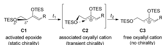
Scheme 4. Possible electrophilic species in the (4+3) cycloaddition.
