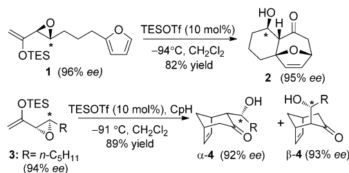
Scheme 2. Diastereoselective (4+3) cycloadditions. TES = triethylsilyl, Tf = trifluoromethanesulfonyl.
